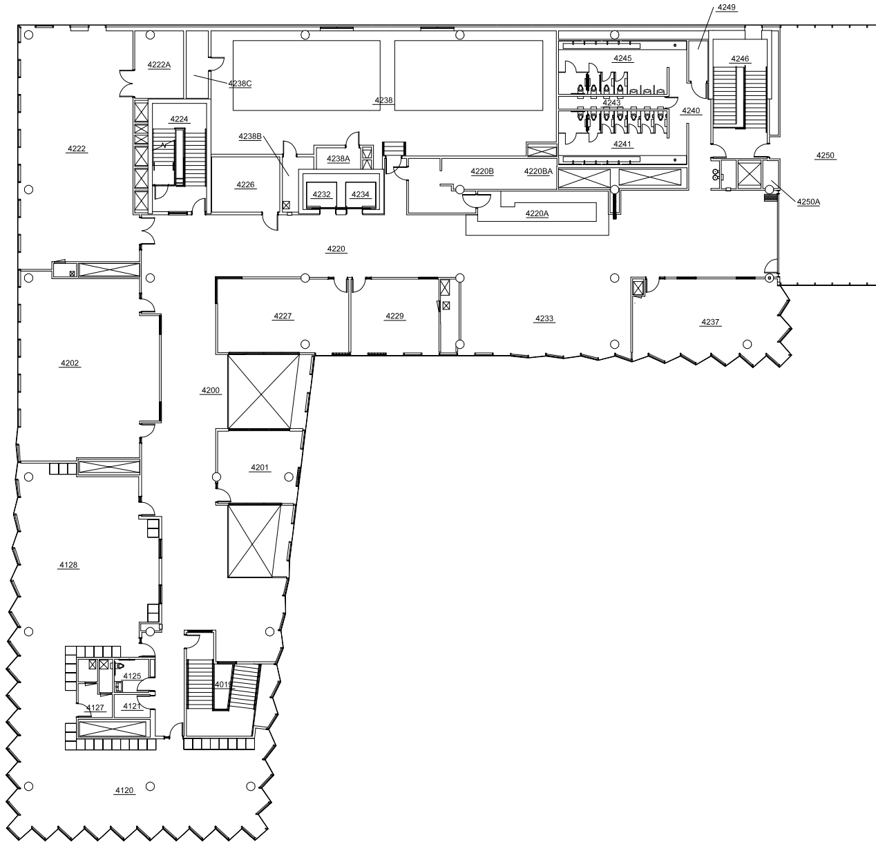
FOURTH FLOOR PLAN
